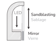
Section profile Section profil
